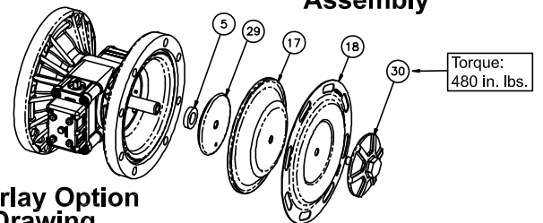
Fluid End Section Assembly
