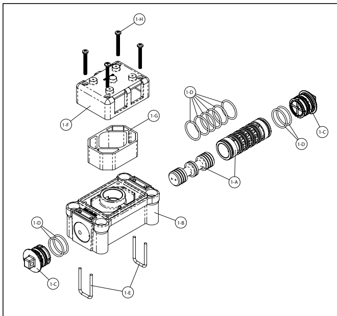
Air End Section Assembly
