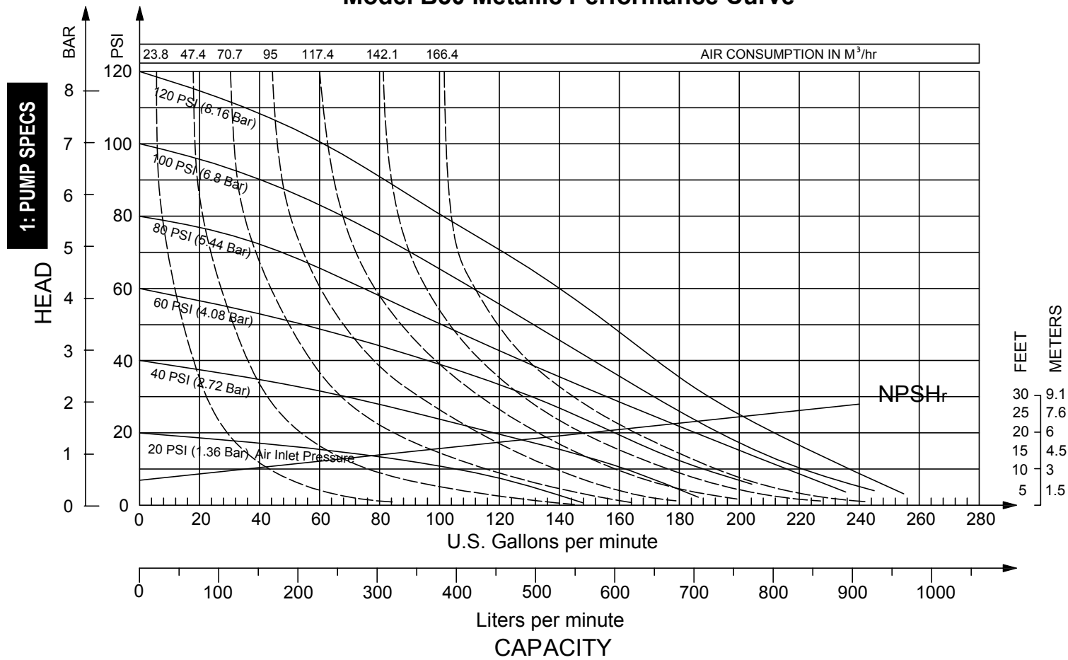
Model B30 Metallic Performance Curve
